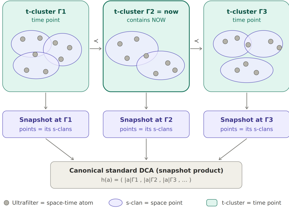
Figure 2: The three kinds of abstract points in a dynamic contact algebra (DM-III.3). Ultrafilters act as space-time atoms. They fall into disjoint t-clusters, which serve as time points and are ordered by \prec , inherited from the precedence relation \mathcal{B} ; the cluster containing NOW is now . Within each t-cluster, s-clans (which may overlap, since spatial contact is not transitive) serve as the space points of that moment's coordinate contact algebra. The original algebra embeds into the product of these snapshots by sending each region a to its vector of equivalence classes.
