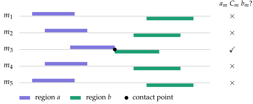
Figure 1: A film strip for two dynamic regions a and b across five moments; each row is a snapshot, drawn here in one spatial dimension. The regions touch only at m_3 . Hence a C^\exists b (equivalently a C^s b ) holds, witnessed by m_3 , while a C^\forall b fails, witnessed by any other row; a C^t b holds because both regions exist together at every moment. Reordering the rows changes none of these verdicts, but it can change verdicts of precedence, which is the only relation in the list that depends on \prec .
